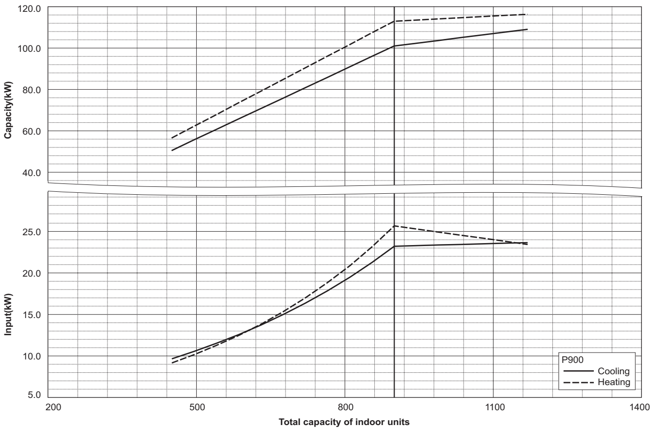
PQHY-P900YSHM-A
